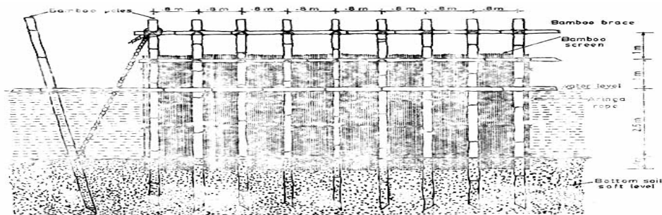
Fig.58: Flexible Enclosures
