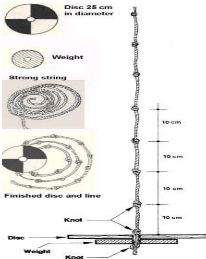
Fig. 15: Preparation of secchi disc
