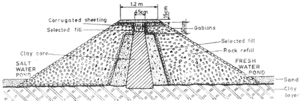
Fig.56: Embanked pens
